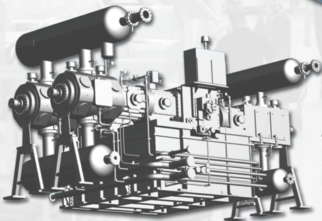
3D Model of Four-throw Compressor
