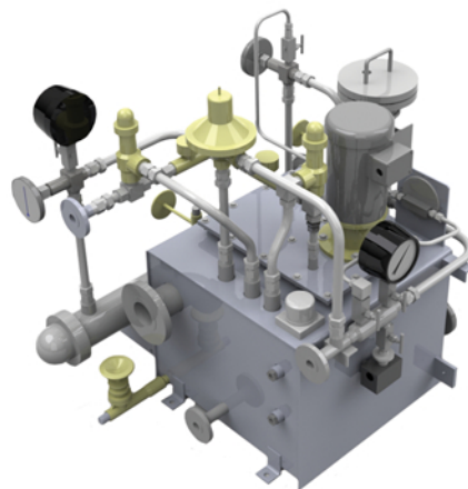
Lube Oil Systems
