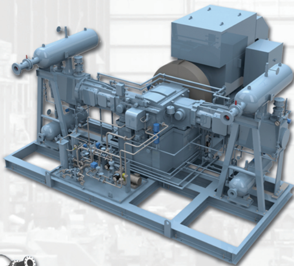
3D Model of Two-throw Compressor
